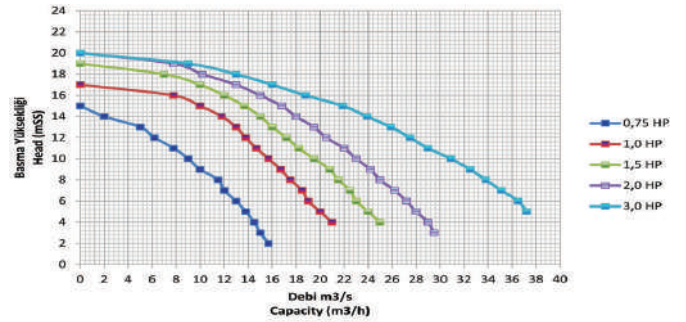
DEBİ DİYAGRAMI
